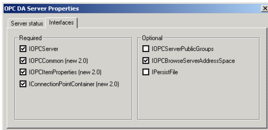
Server Properties Dialog Box: Interfaces Tab
