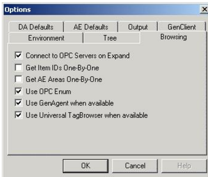
Options Dialog Box: Browsing Tab
