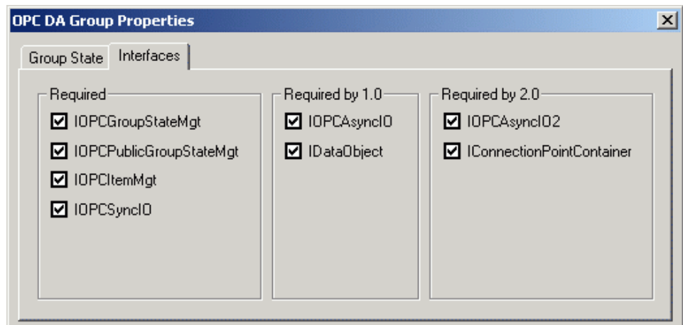
Group Properties Dialog Box: Interfaces Tab
