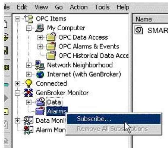
Subscribing to an OPC AE Server
