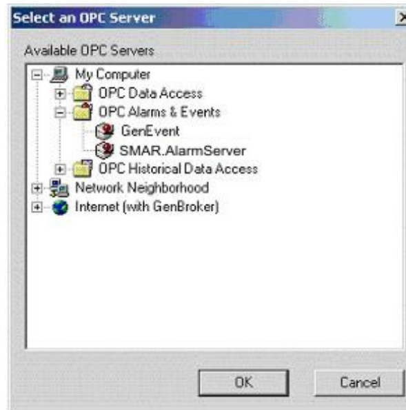
Selecting an OPC Server
