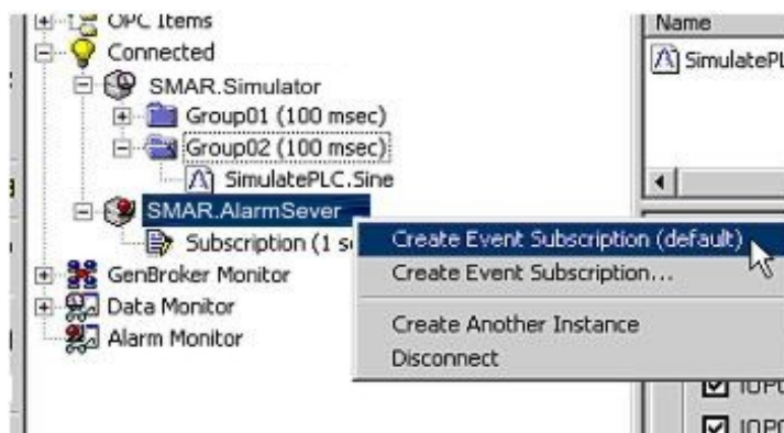
Creating an Event Subscription
