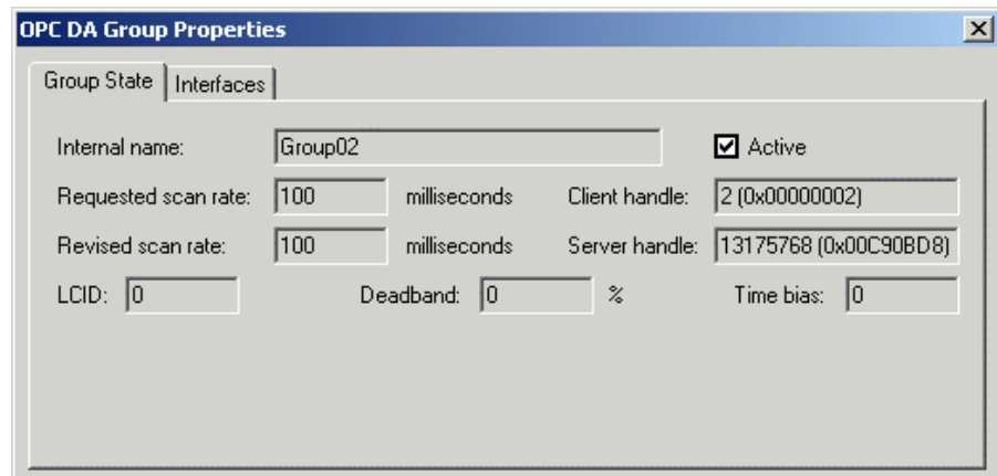
Group Properties Dialog Box: Group State Tab
