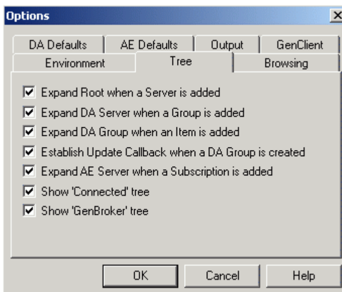
Options Dialog Box: Tree Tab
