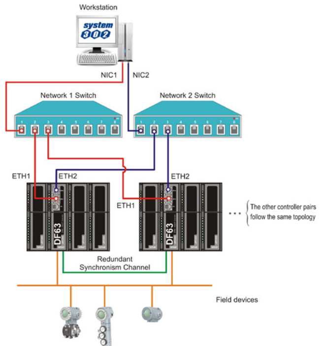
Basic architecture for DFI302 controllers with two Ethernet ports
